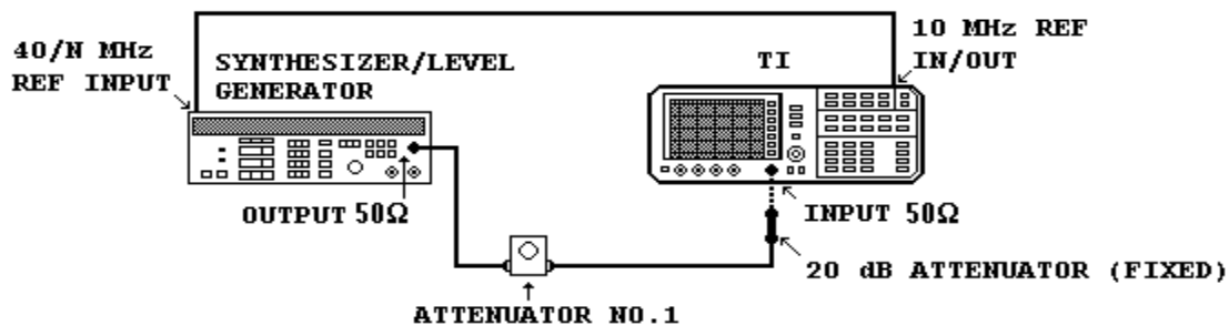
Figure 2. Input attenuator accuracy (50 MHz) - equipment setup.
