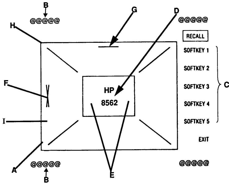
Figure 1. Crt adjustment pattern.
